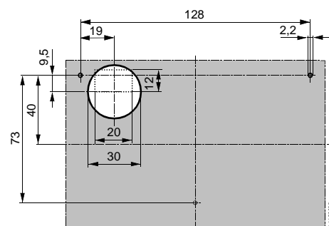
Drilling template for front mounting
