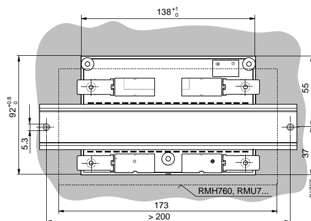
Control panel cutout (with controller/RMB795/RMS705 mounted at the rear)
