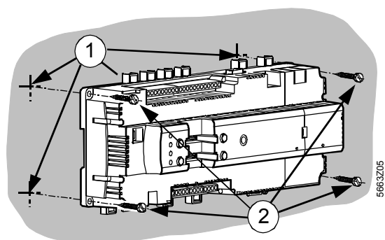
Screwed-on mounting
